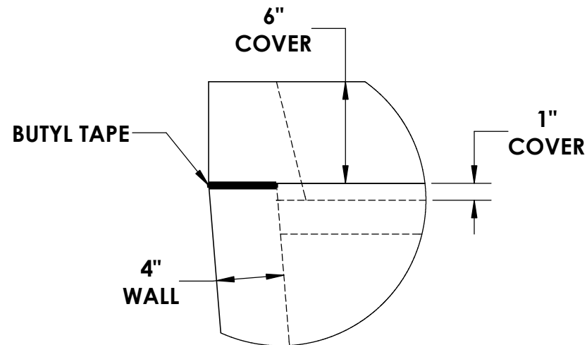
JOINT DETAIL A
